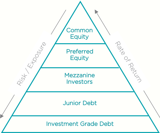
Traditional State
